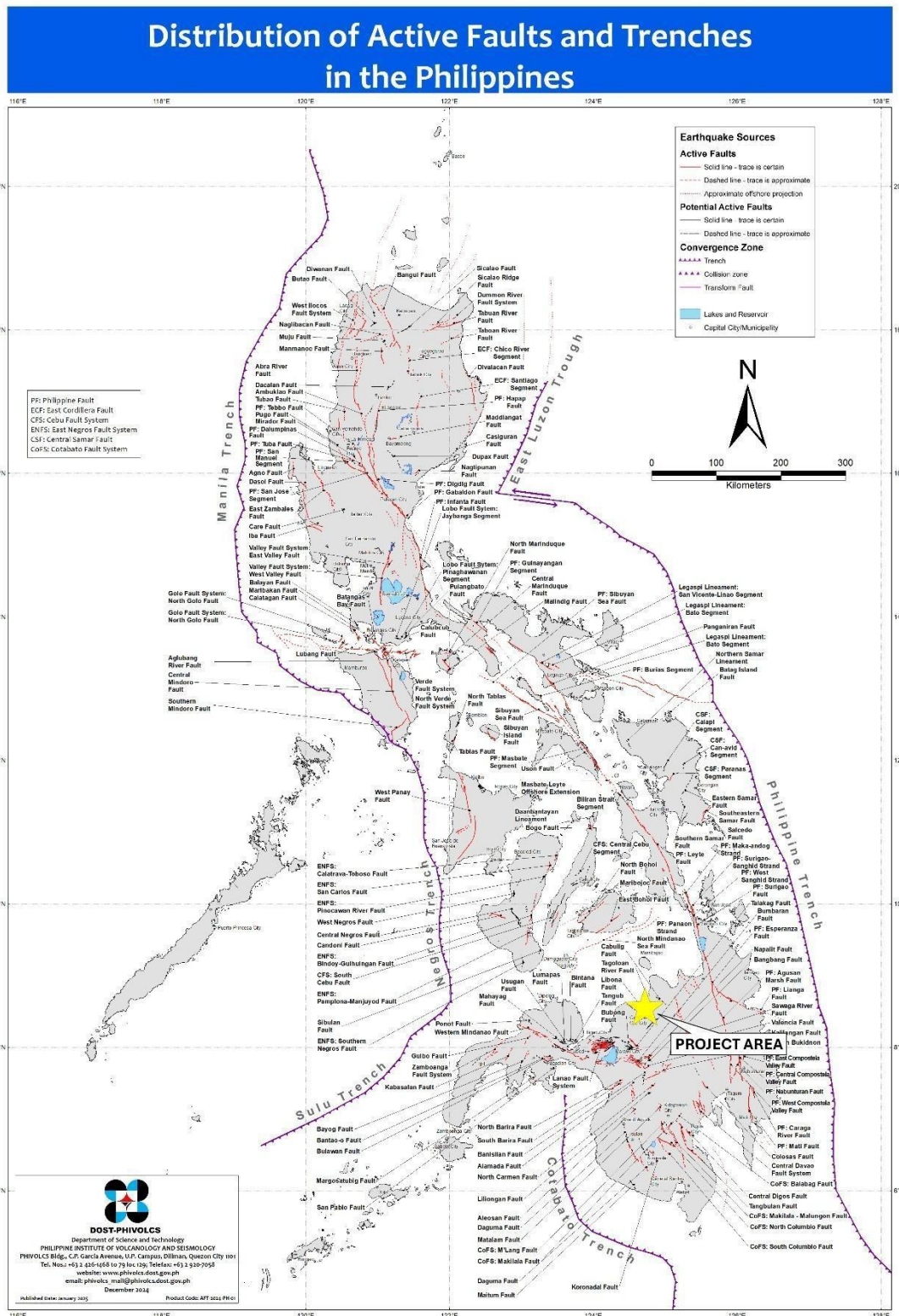
Figure 7-9. Active Faults and Trenches Map in Relation to the Project Site
