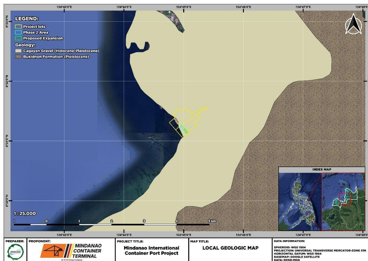
Figure 7-8. Local Geologic Map of Project Site
