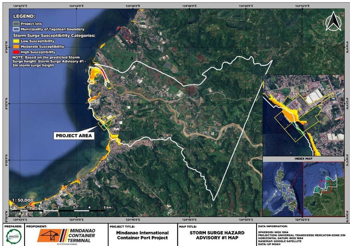
Figure 7-16. Storm Surge Advisory No. 1 Hazard Map in Relation to the Project Site
