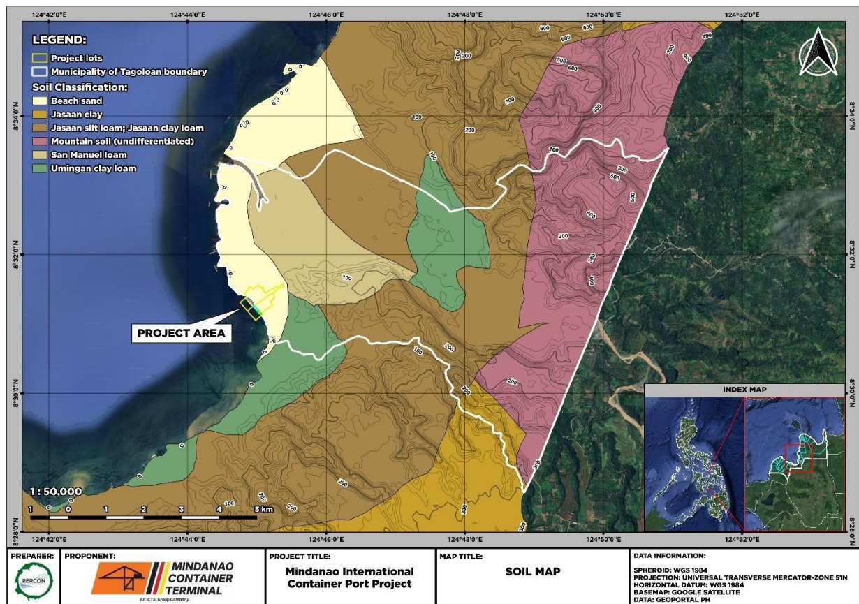
Figure 7-17. Soil Map of the Project and Vicinity
